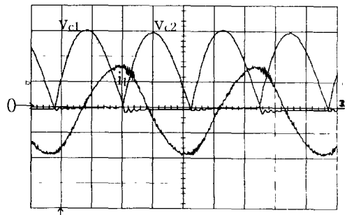
50(v)/div, 5(A)/div, 2(µs)/div (a) f_o=90[kHz]
